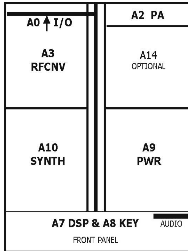
BOTTOM VIEW
