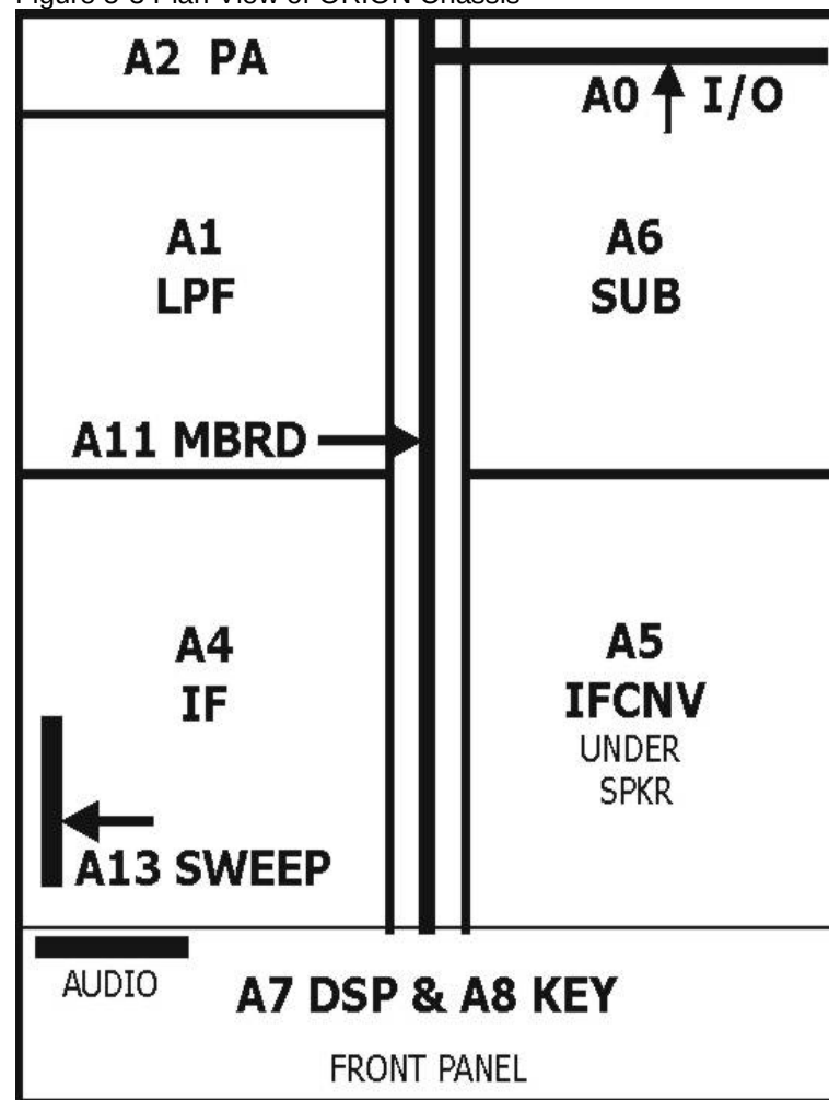
TOP VIEW
