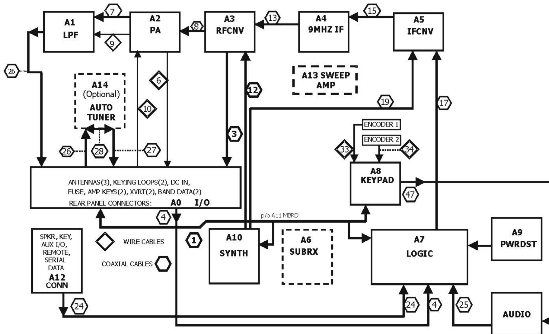
Figure 5-6 Transmit Signal Path
