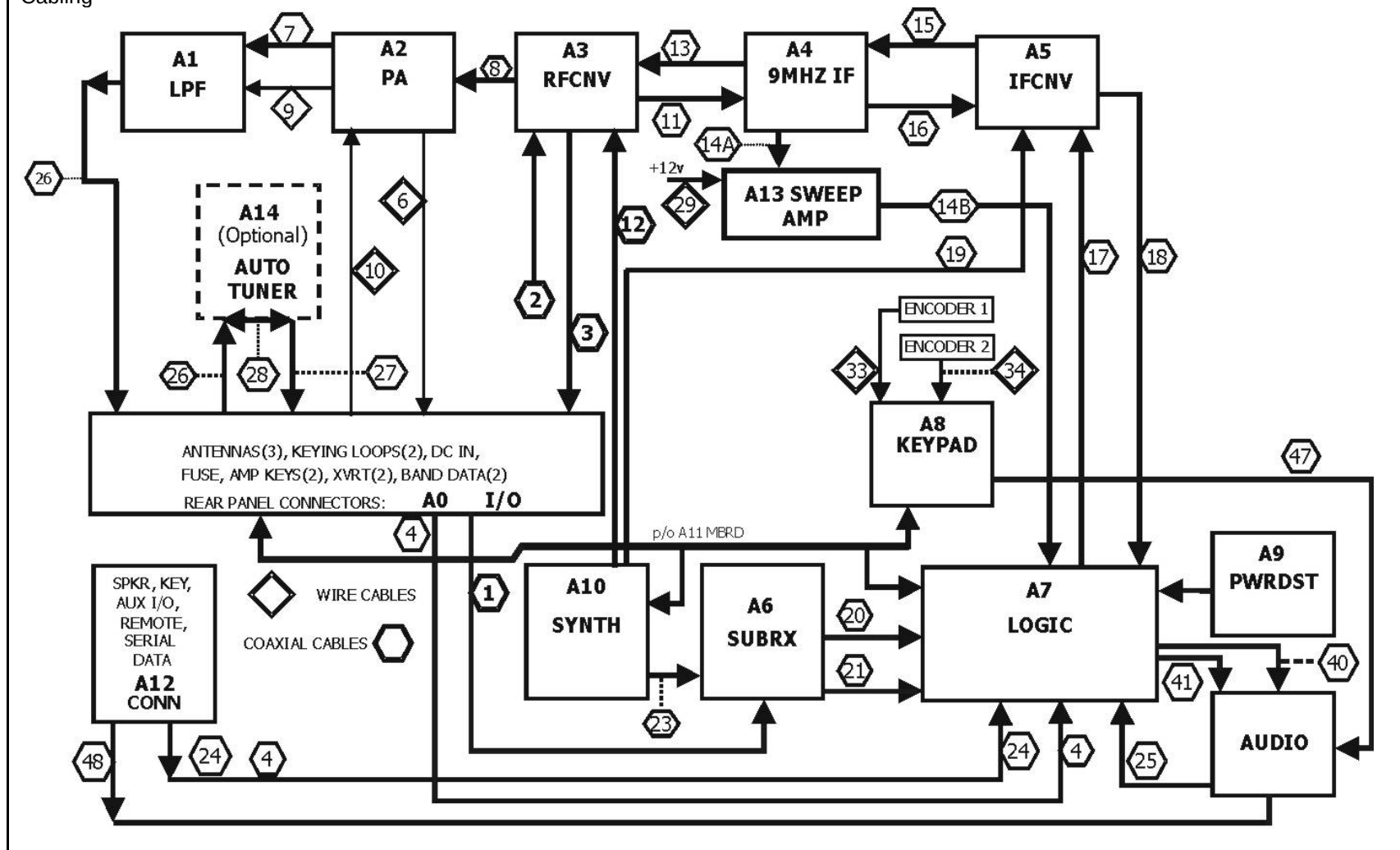
Figure 5-2 Subassembly Cabling
